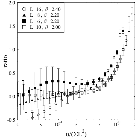
Figure 7. The ratio of Eq. (14) versus u/(\Sigma L^2) for four different parameter sets.
