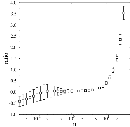
Figure 5. The ratio defined in Eq. (14) versus u for the data obtained on a 10^4 lattice using \beta = 2.0 .
