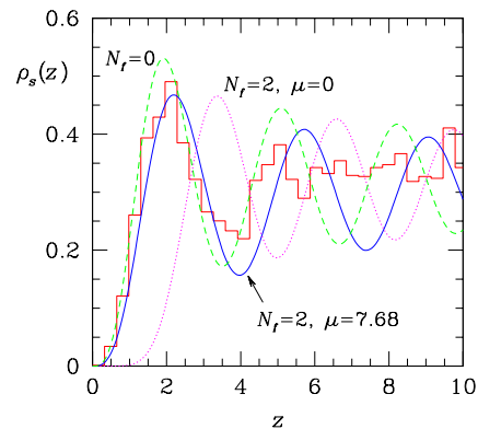
Figure 3. Distribution of the smallest eigenvalue (top) and microscopic spectral density (bottom) for the simulation parameters indicated above the figures. The histograms represent the lattice data. The solid curves are the RMT results computed with the appropriate value of the rescaled quark mass \mu . The dashed and the dotted curves are the RMT results computed in the quenched approximation and in the chiral limit, respectively.
