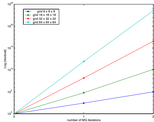
Fig. 1 Example 1: Divergence of the multigrid solver M(R^{lin}, P^{lin}) .
