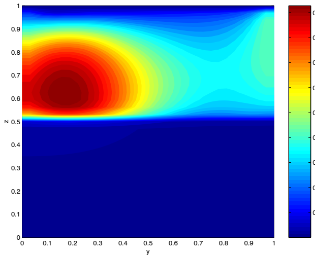
Fig. 6 Example 2: Pressure of the fluid in the cross-section x = 0.53125 .
