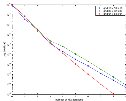
Fig. 4 Example 2: Convergence of the multigrid solver M(R^{od}, P^{od}) .
