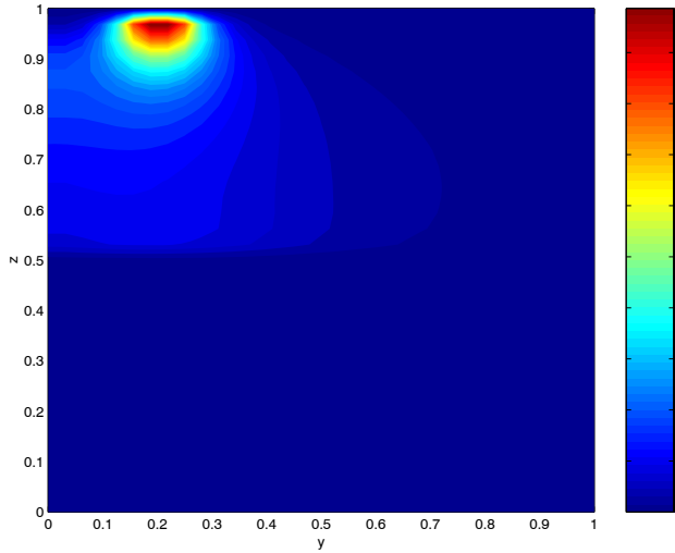
Fig. 5 Example 2: Pressure of the fluid in the cross-section x = 0.1875 .
