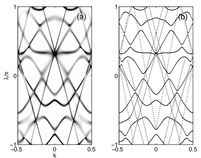
FIG. 1. Wigner delay time as a gray scale map (a) and the real part of the complex quasienergy spectrum (b) [for each k first 13 most stable states is plotted]. The system parameters are \omega = 10/6 , \epsilon = F_\omega/\omega^2 = 1.5 , \hbar = 0.5 , and F = \hbar/T_\omega \approx 0.13
