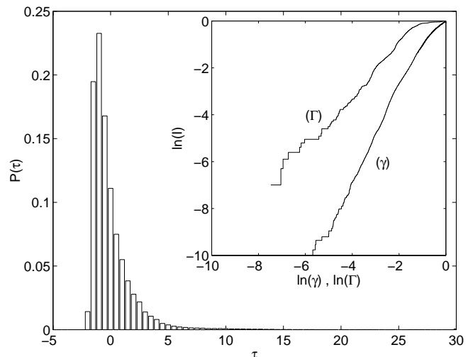
FIG. 2. The distribution of the Wigner delay time. The insert shows integrated distributions of inverse delay time \gamma = 1/\tau and resonance width \Gamma .
