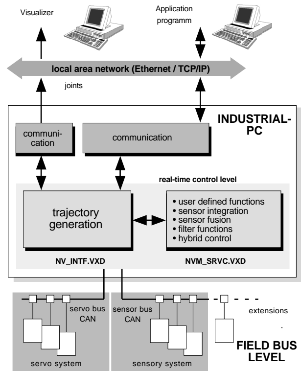
Figure 3: Structure of the PC-based robot control system
