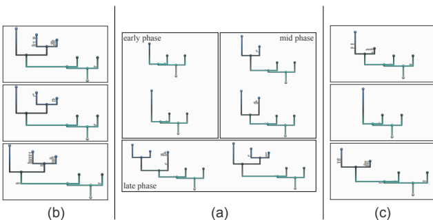
Fig. 10: Six member trees from the heated cylinder ensemble (a) with several barycenters. The six example members come from three different phases of one single run. The barycenters on the right (c) were computed on a consecutive subsequence of a single run, whereas the barycenters on the left (b) were computed on one fixed time step from the late phase for each run. The top row barycenters in (b) and (c) were computed using the path mapping distance and the typical mean method. The center row barycenters are based on the path mapping distance in the median variant. The bottom row barycenters are the Wasserstein barycenters.
