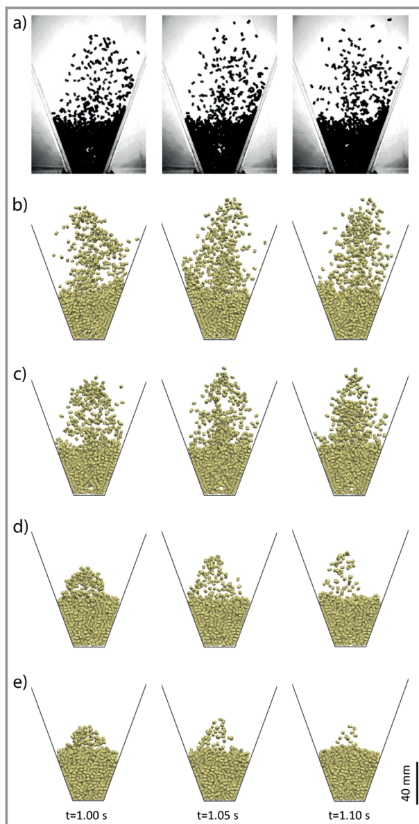
Figure 3. Snap shots of the fluidization of the cylindrical particles for a gas inlet velocity of 1.44 \text{ m s}^{-1} in a) the experiment and the simulations with the drag model according to b) Sanjeevi et al. [34], c) Hölzer and Sommerfeld [36], d) Bagheri et al. [46], e) Dioguardi et al. [47].
