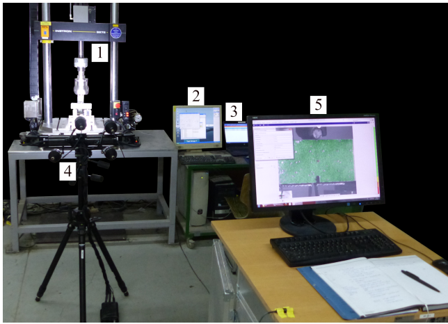
FIGURE 4 Experimental setup: 1 + 2 = testing machine, 3 = PC for the clip gauge, 4 = DIC, 5 = control of the DIC. DIC, digital image correlation
