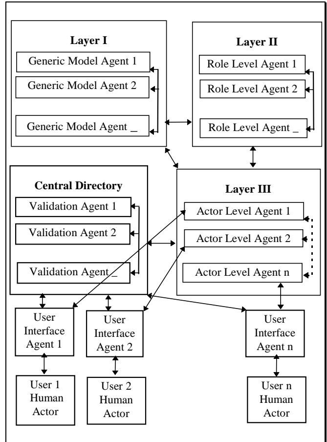
Fig. 7. - The layered multi-agent architecture of the co-ordination mechanism.
